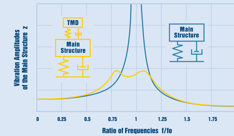
Vibration of the Main Structure
