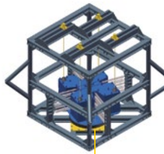
Horizontal TMD
