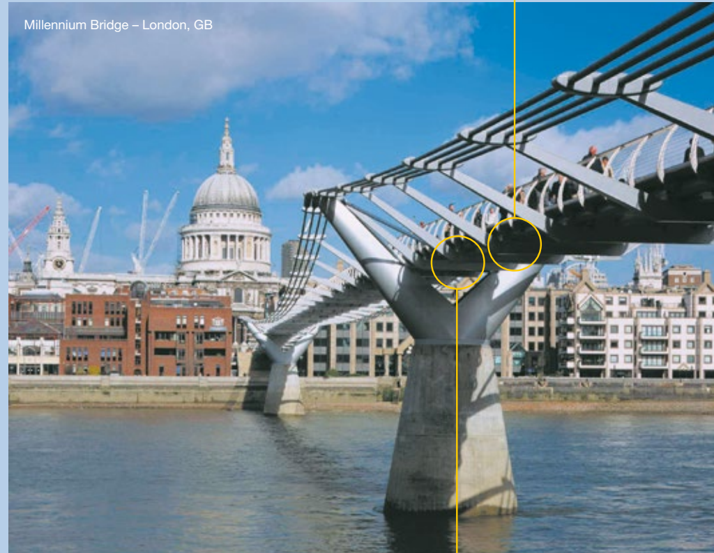
Vertical TMD
