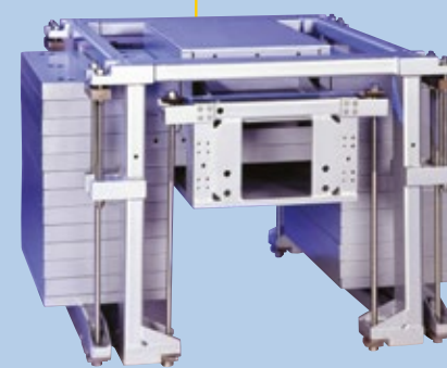
Horizontal TMD
