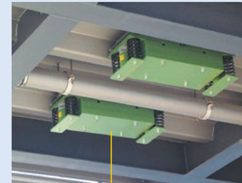
Vertical TMD
